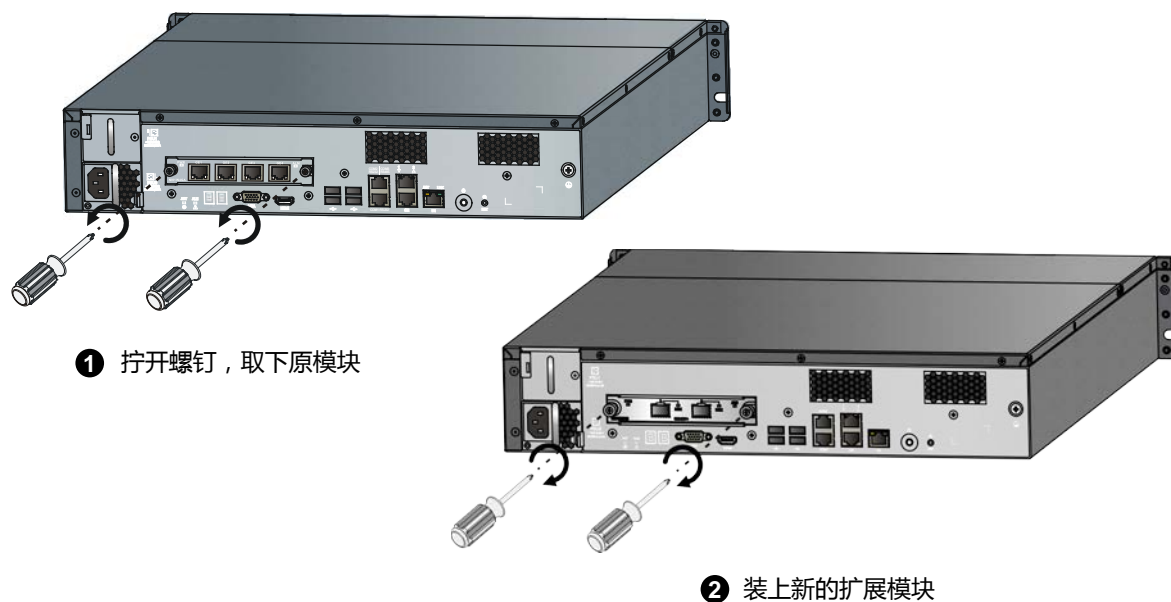
图2-10 更换扩展网卡
